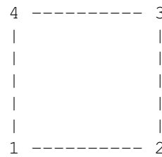
ESMF_MESHELEMENTTYPE_QUAD
