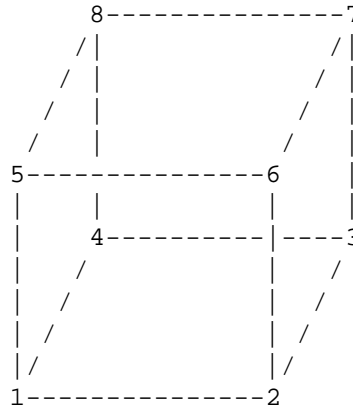
ESMC_MESHELEMENTTYPE_HEX
